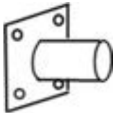
WMT Wall Mount Tenon (Steel) Use for mounting fixtures with Slip Fitter to Wall. Tenon is 2.38" OD x 4". Bronze; Optional Custom Colors.
