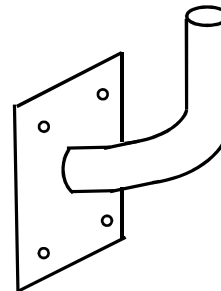
WMPP Wall Mount Parapet (Aluminum) Mounts to building Parapet; 2.38" OD x 4" Tenon. Bronze; Optional Custom Colors.
