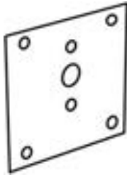
WMP Wall Mount Plate (Steel) Use for mounting fixtures with Arms to Recessed Box. Bronze; Optional Custom Colors.
