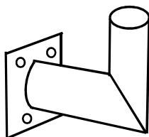
WMT Wall Mount Tenon (Steel) Use for mounting fixtures with Slip Fitter to Wall. Tenon is 2.38" OD x 4". Bronze; Optional Custom Colors.
